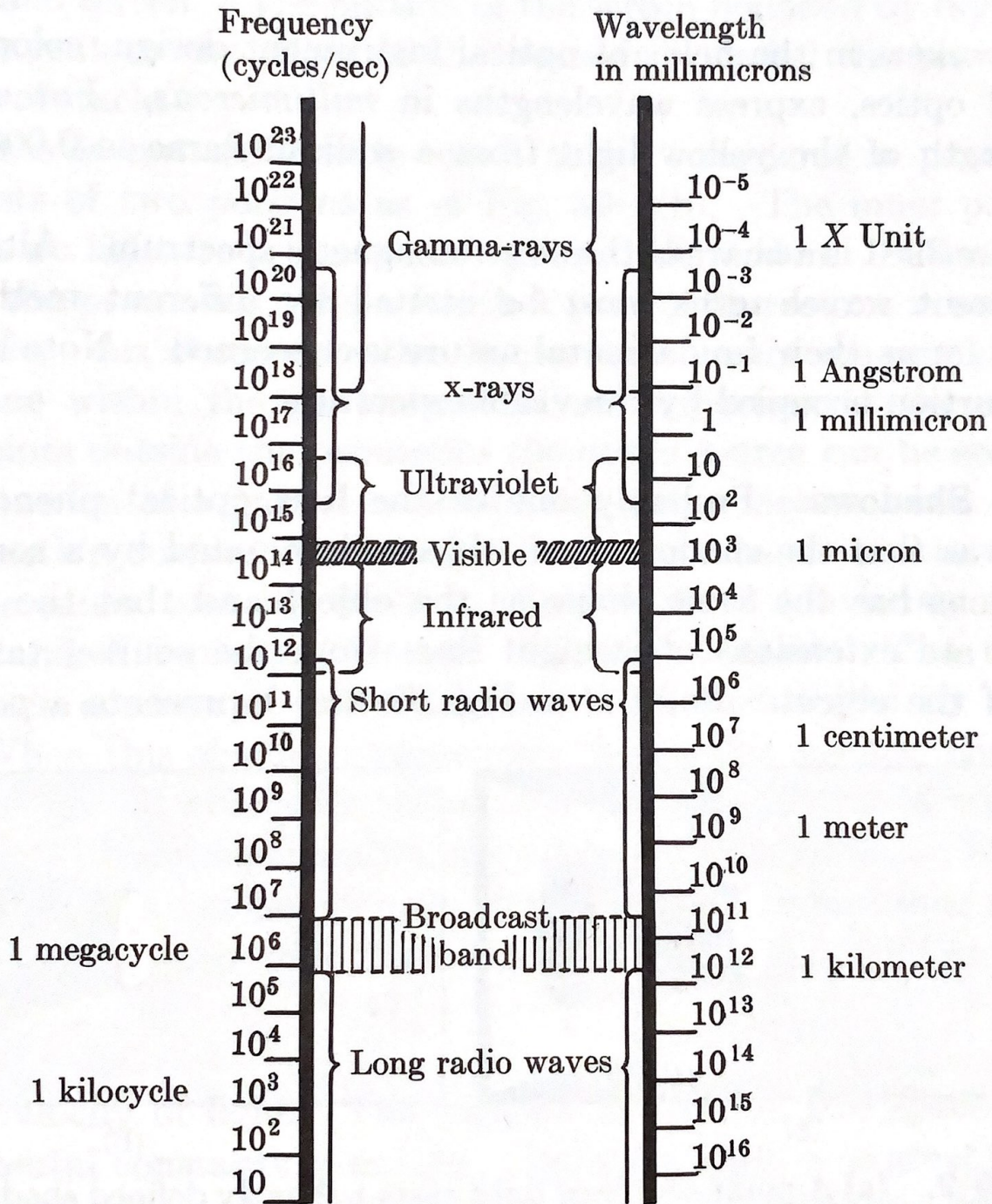
Fig. 39-1. A chart of the electromagnetic spectrum.
